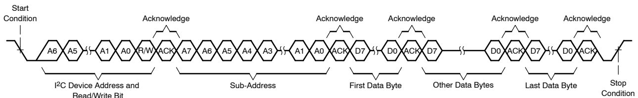
Figure 4-3. Multiple-Byte Write Transfer
