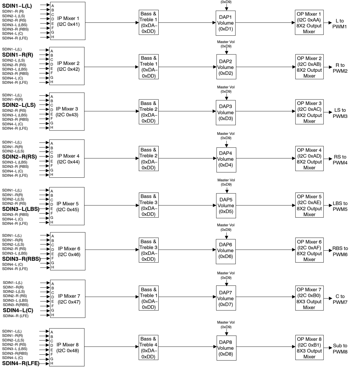
Figure 1-4. TAS5028A DAP Architecture With I 2 C Registers (Fs ≤ 96 kHz)
